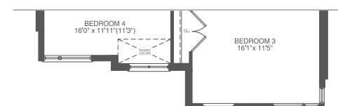
SECOND FLOOR ELEVATION C 3437 sf
