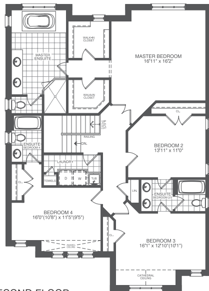
SECOND FLOOR ELEVATION A 3102 sf
